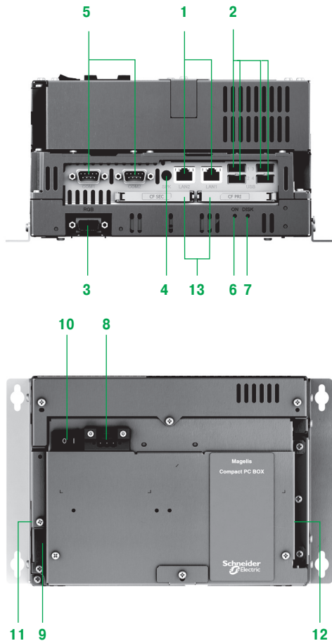
Magelis Compact PC BOX: MPC KNO 2NAX 00N
